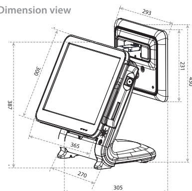
Dimension view
